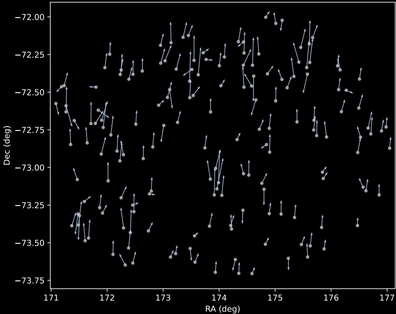
GALAH DR4 Cluster 1 Proper Motion Vectors (n=165)
