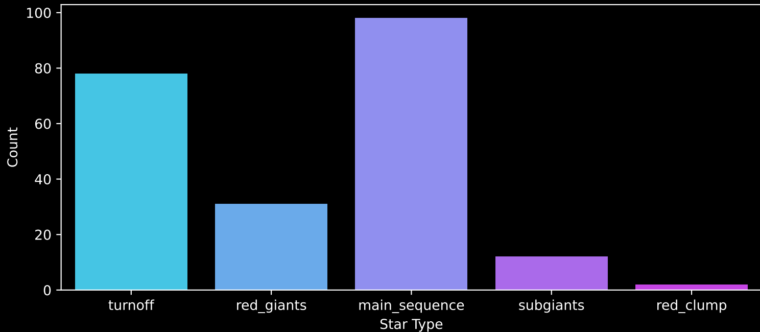
GALAH DR4 Field: [548] Count plot of Star Type
