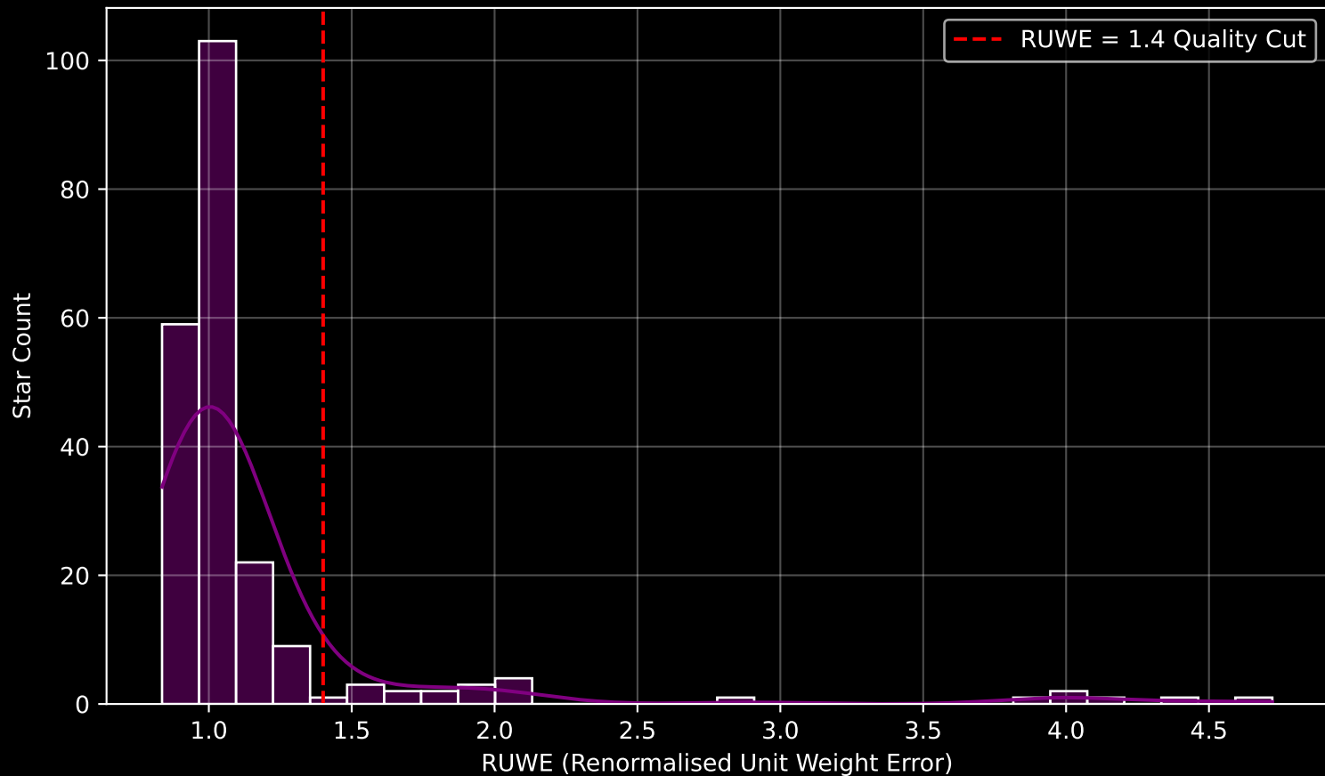
GALAH DR4 Field [548] RUWE Distribution (n= 215)
